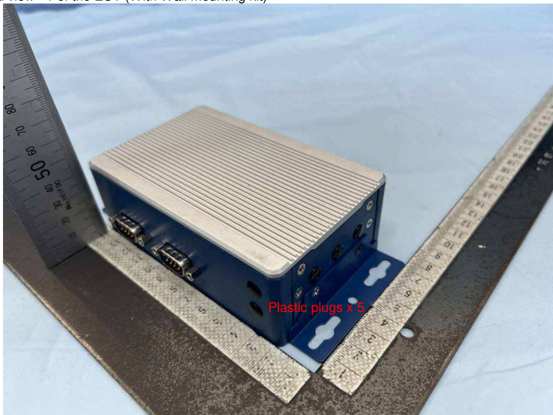
General view - 1 of the EUT (With Wall mounting kit)
