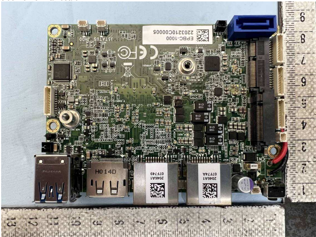
Bottom side view of mainboard
