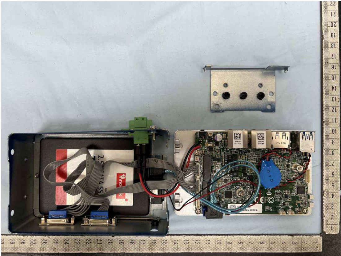
Internal view - 1 of the EUT
