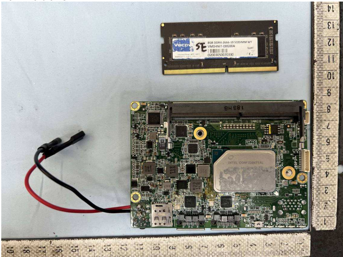
Internal view - 4 of the EUT
