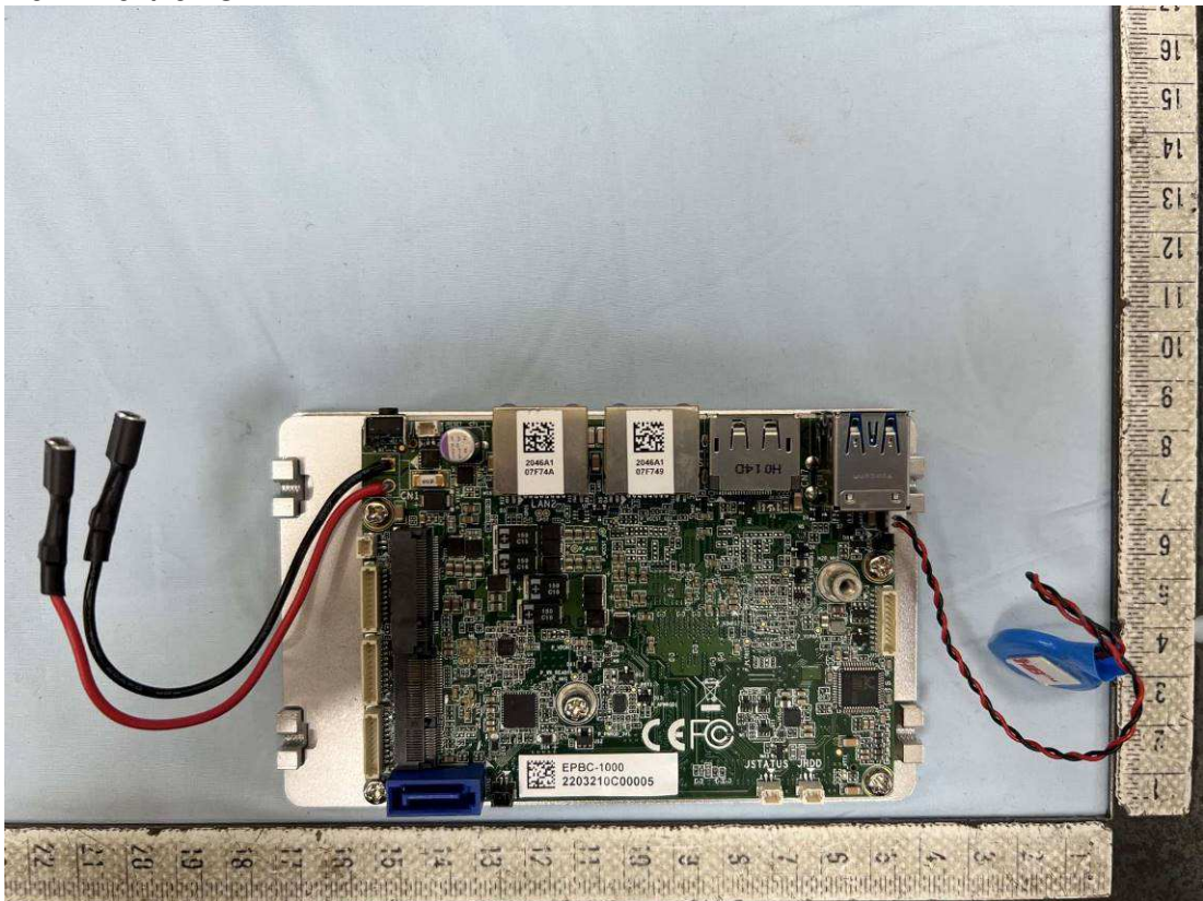
Internal view - 2 of the EUT
