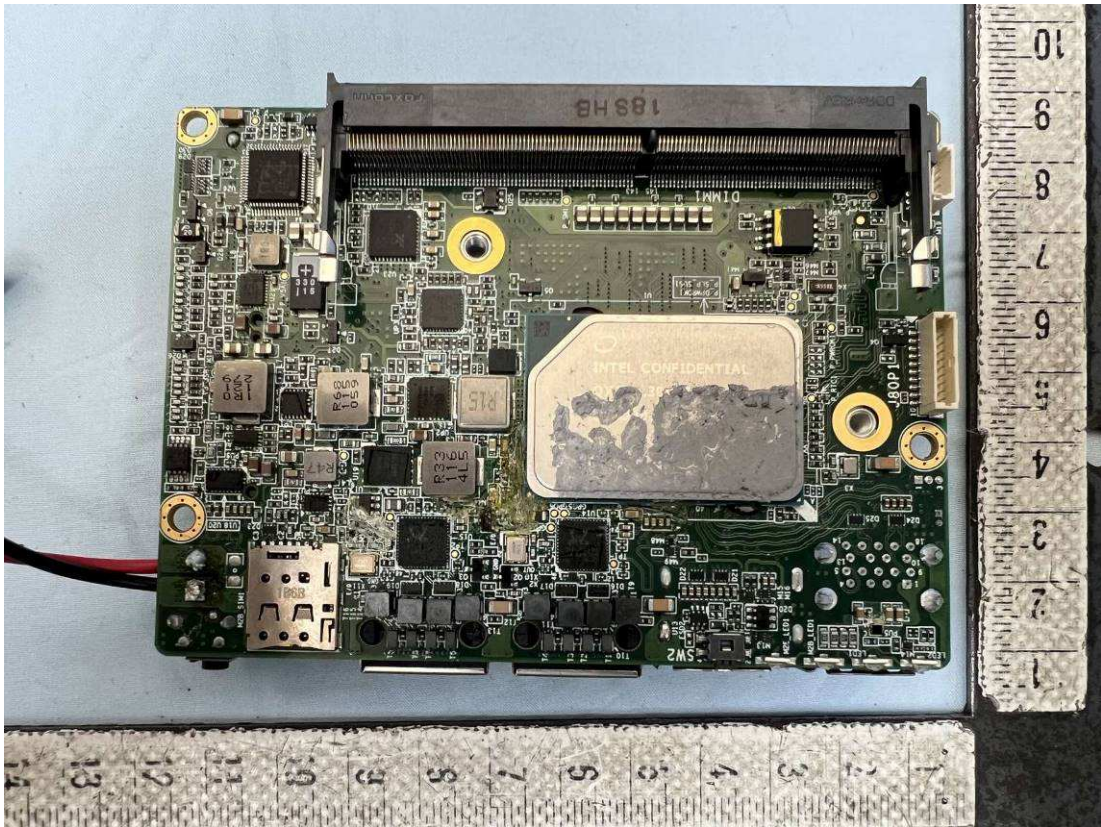
Top side view of mainboard
